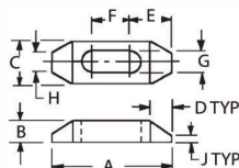
Plain Clamp
